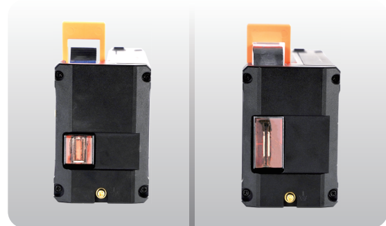
Convertible between 0.5"/1" cartridges by replacing printhead plates
